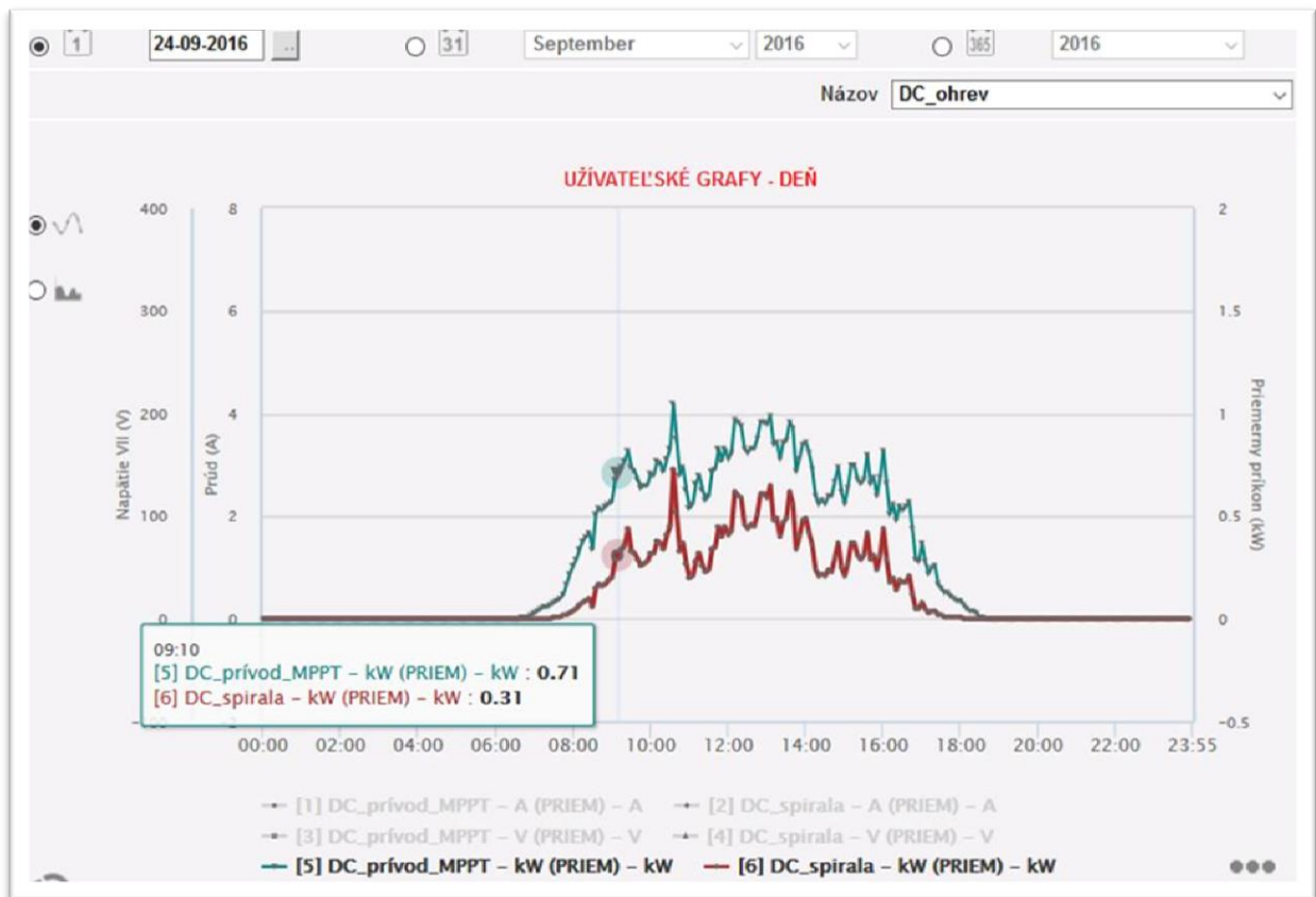
Maximum power point tracking - MPPT
